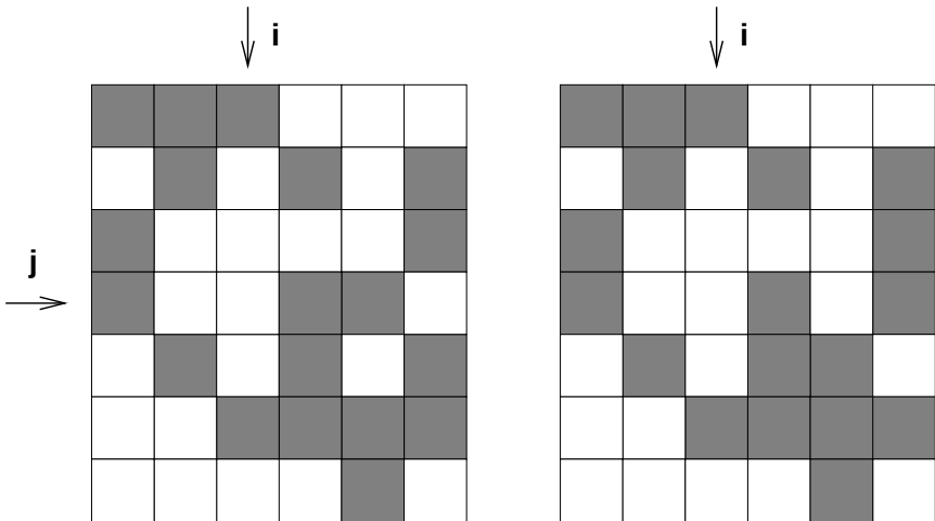
Fig. 1. One step equivalence by crossing-over
